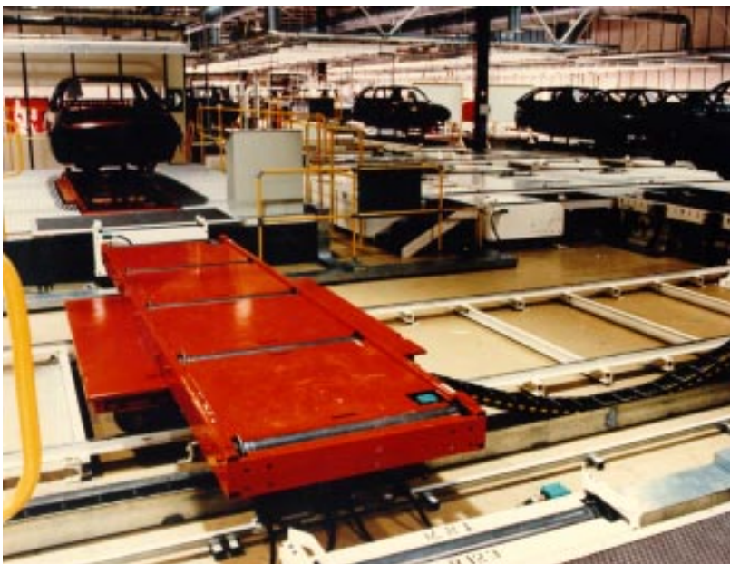
Above: Accumulation or Buffer Floor Skid Conveyor Systems have a chain or belt powered track on one side and a supporting idler roller track on the other side of the conveyor.
